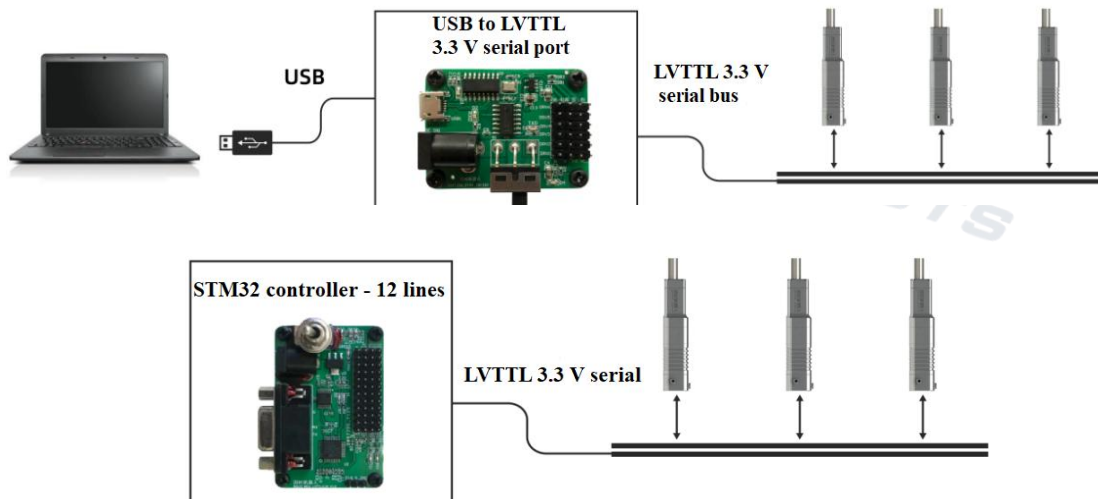
Figure 5: Communication Mode Diagram
